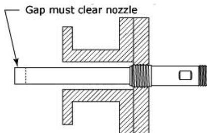
Figure 5 Nozzle Mounting
