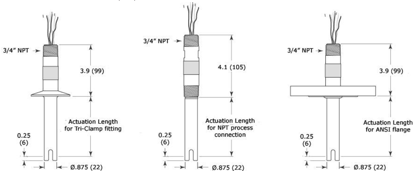
Model U002/3 with Sanitary flange
