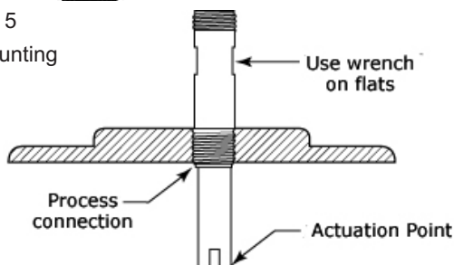
Figure 6 Vertical Mounting
